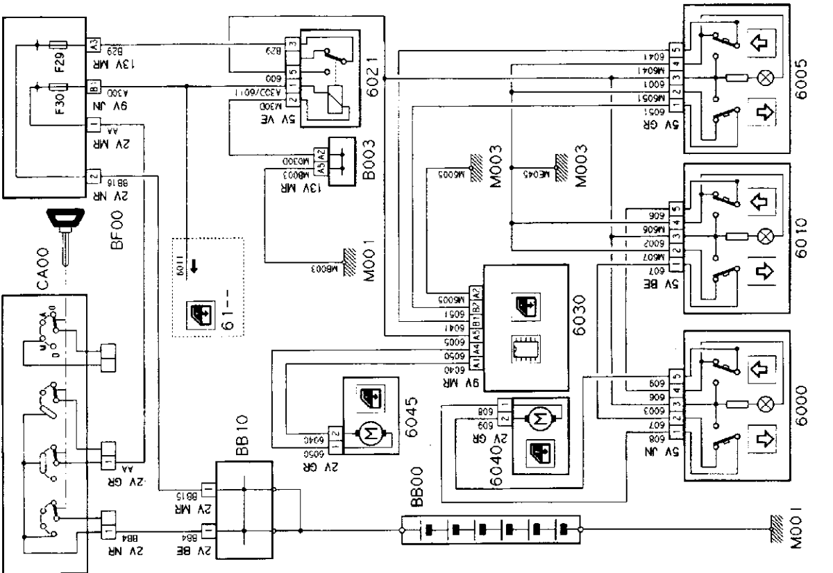
Front electric windows
