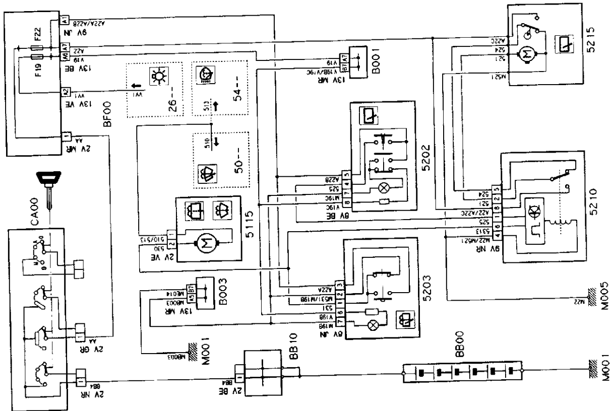
Typical rear screen wash/wipe
