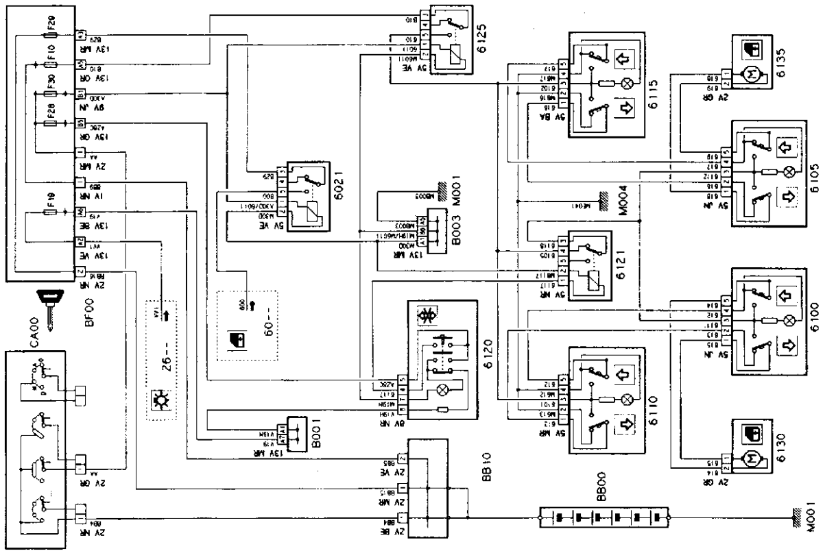
Rear electric windows
